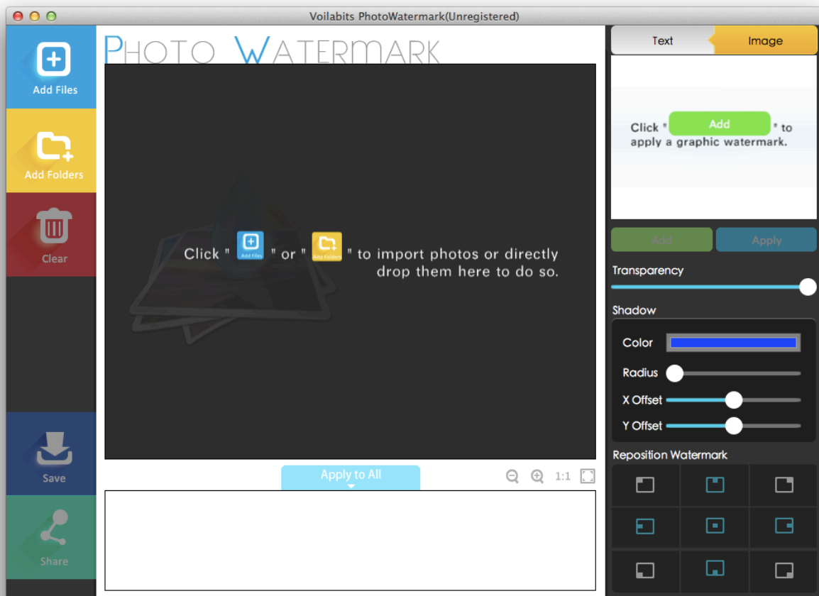
Figure 1: Main Interface
